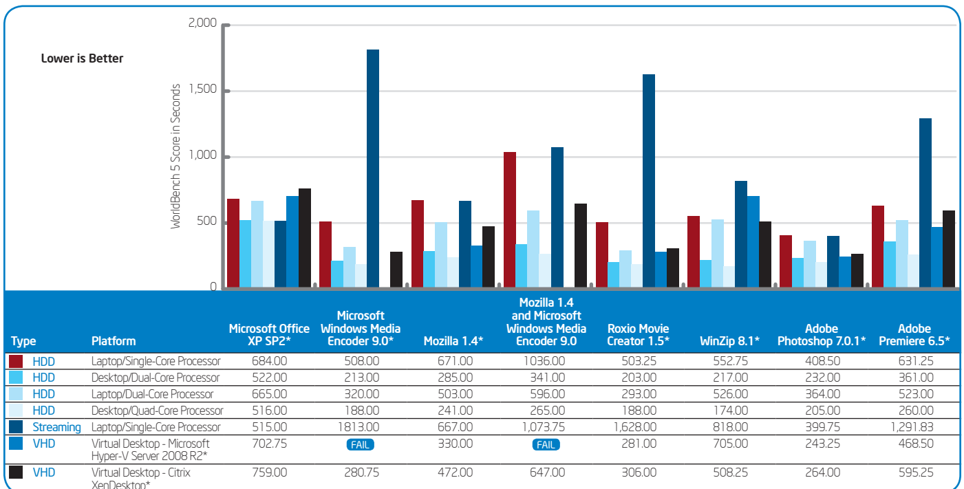
Figure 6. WorldBench 5* scores for streaming, virtual hosted desktop (VHD), and traditional PCs. Tests conducted by Intel using WorldBench 5. WorldBench is a trademark of International Data Group, Inc. Test results have not been verified by PC World, and neither PC World nor International Data Group, Inc. makes any representations or warranties as to the accuracy of the test results.
