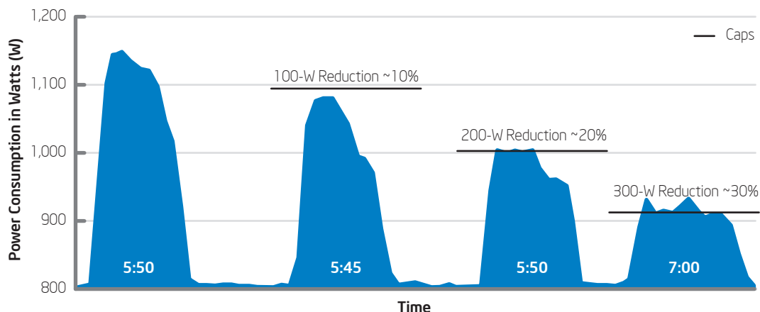
Figure 1. We used capping to reduce server power consumption by approximately 20 percent when running an I/O-intensive workload, without impacting runtime.
