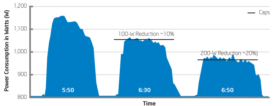
Figure 3. Effects of capping on runtime of CPU-intensive workloads. Reducing power consumption by 20 percent resulted in an 18 percent increase in runtime.
